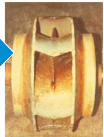
Coated Impeller After 7 Years Service
